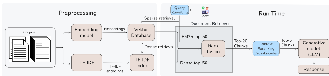
Gambar IV.6 Diagram Alur Pipeline Konfigurasi Query Rewriting dan Context Reranking
