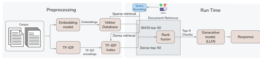
Gambar IV.4 Diagram Alur Pipeline Konfigurasi Query Rewriting
