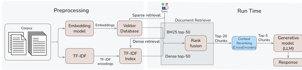
Gambar IV.5 Diagram Alur Pipeline Konfigurasi Context Reranking
